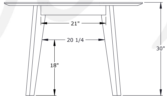
VUE FACE / FRONT VIEW
